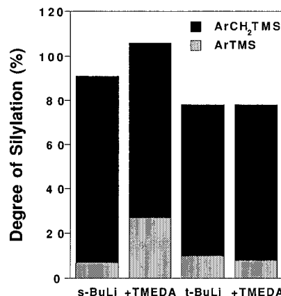
Figure 3. Effect of TMEDA on the reactivity of s - and t -BuLi/ t -PeOK (1/3). Metalation reactions were carried out for 15 min at each temperature in cyclohexane or hexane. (TMS)Cl was used as quencher.
