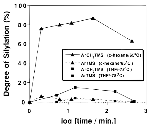
Figure 1. Comparison of the solvents cyclohexane (at 65 °C) and THF (at -78 °C) used in the metalation of poly(IB-PMS). The superbases s -BuLi/ t -PeOK was used in 2-fold excess and the reaction was quenched by addition of aliquots of the reaction mixture to neat (TMS)Cl at given time intervals.
