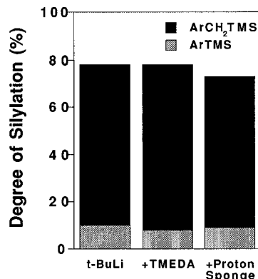
Figure 2. Effect of complexing agents on the reactivity of t -BuLi/ t -PeOK (1/3). Metalation reactions were carried out for 15 min at each temperature in cyclohexane or hexane. (TMS)-Cl was used as quencher.
