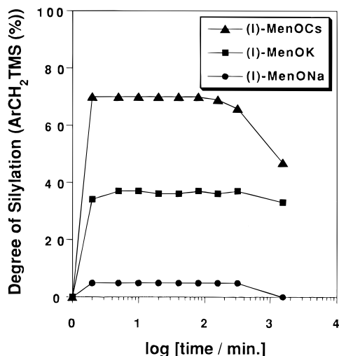
Figure 4. Effect of reaction time on the metalation of poly(IB-PMS) at room temperature using s -BuLi/ M^+ l -(-)-menthoide ( M^+ = \text{Na, K, Cs} ) carried out in cyclohexane. (TMS)Cl was used as quenching agent. Aliquots of the reaction mixtures were taken at time intervals and added to neat (TMS)Cl.
